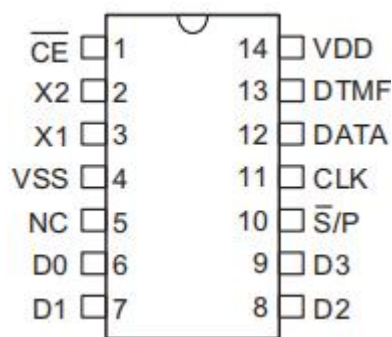
HT9200B SOP-14
